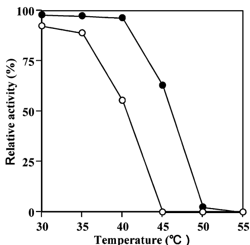
Fig. 1. Effects of temperature on the stability of the wild-type and mutant BFB40 enzymes. The remaining activities were assayed under the standard condition after the purified enzymes had been incubated at various temperatures for 5 min, and expressed as a percentage of the activity of each untreated enzymes. Symbols: (○) wild-type; (●) BFB40.
